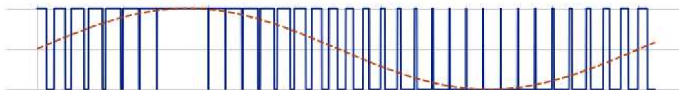
Figure 2.10 – A PWM signal in blue, with the dashed line showing its approximate value
