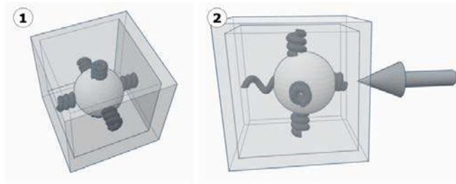
Figure 12.17 – Accelerometer concept – mass with springs
