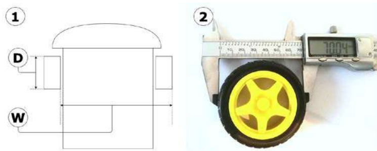
Figure 11.11 – Measuring the wheel
