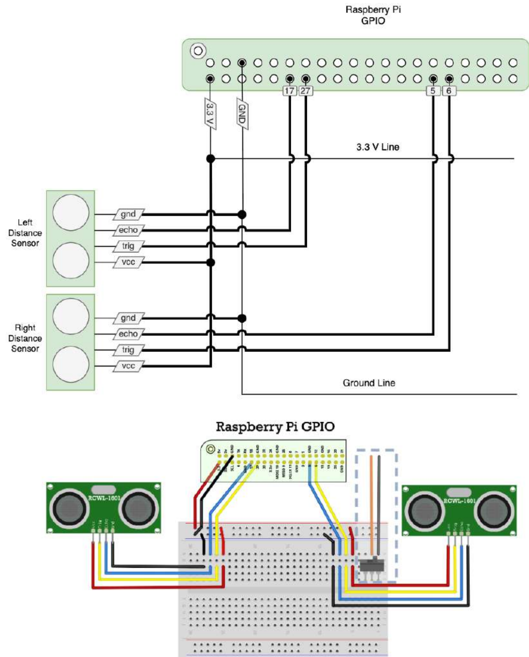
Figure 8.15 – Sensor wiring diagram
