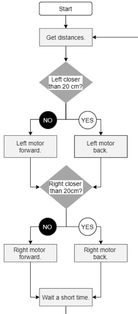
Figure 8.19 – Obstacle avoidance flowchart
