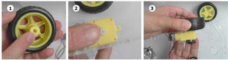
Figure 6.26 – Fitting the wheels
