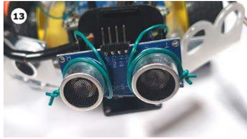
Figure 10.21 – The sensor temporarily secured to the pan-and-tilt head
