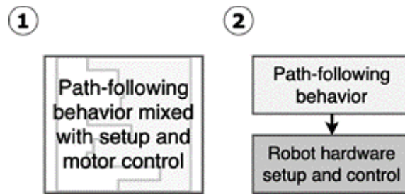
Figure 7.6 – Software layers
