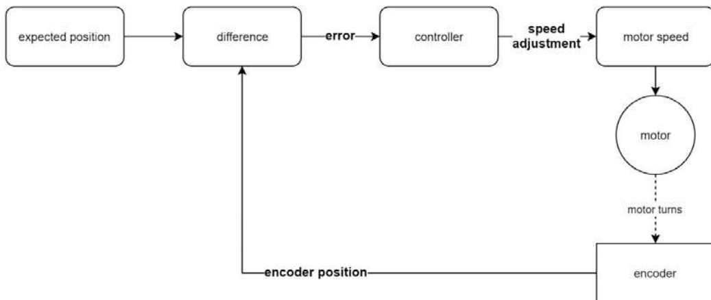
Figure 11.12 – Closed-loop control of a motor's speed
